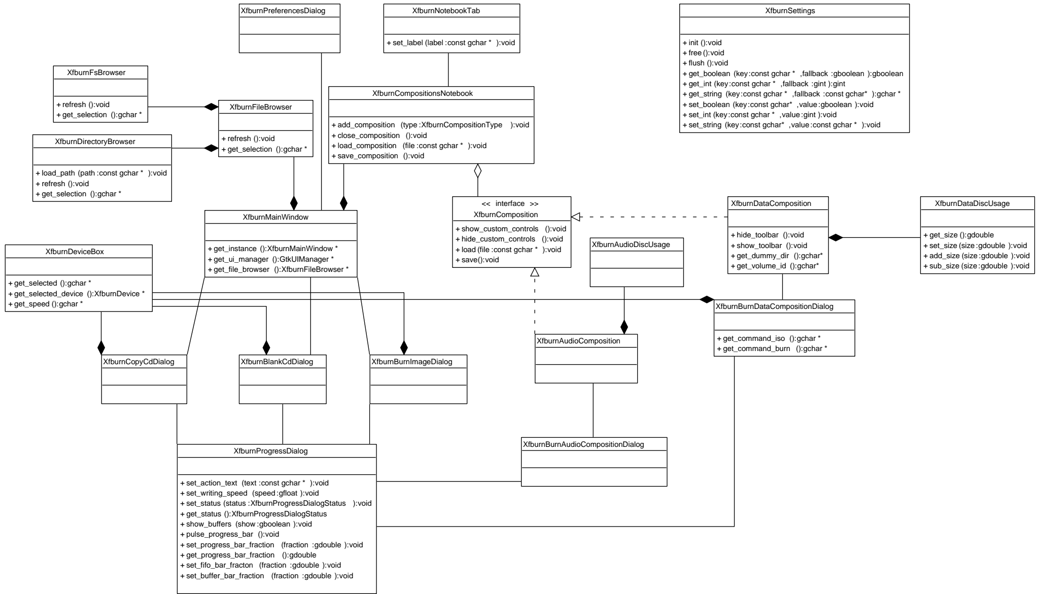
cd: Class Diagram
